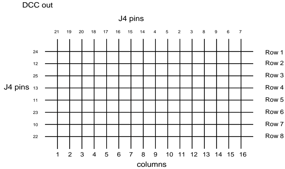
Switch matrix connections from D type.
