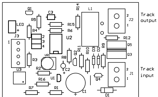
BC01 DCC Block Cutout Rev A
